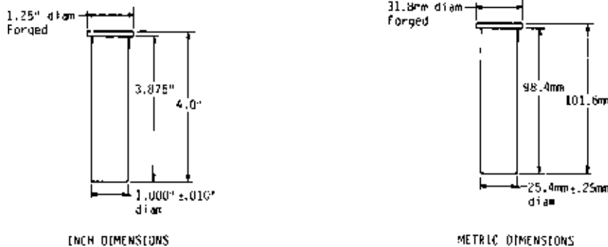
FIG. 2 Preferred Test Specimen
