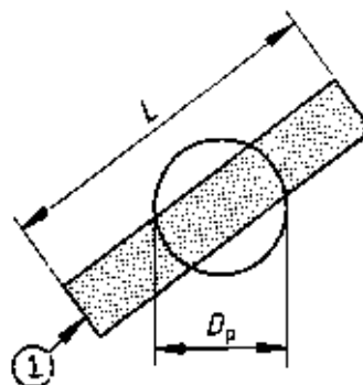
Figure 4 — Extended discontinuity ( L \leq D_p )
